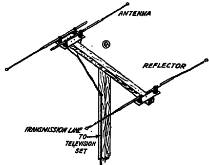
Frequency modulation and television receiving antenna covering the range of 40 to 90 megacycles and employing Q method of coupling between the transmission line and the antenna, and method of mounting this antenna on a mast with a reflector to secure directional characteristics.
